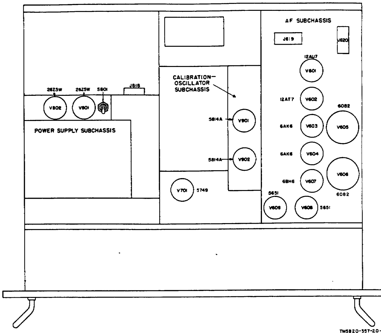
Figure 9. Tube locations, bottom deck.
